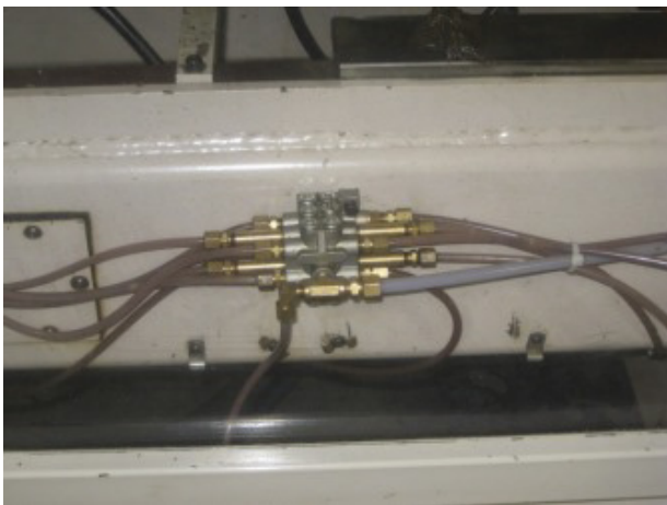
12-Port Distribution Block on Blow Molder
